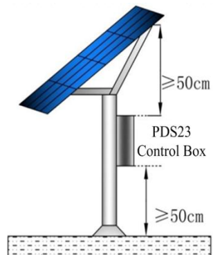
Figure 6 Control Box Location
