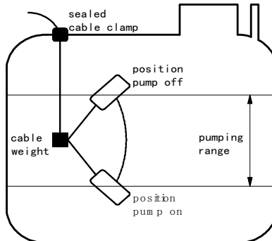
Figure 12 Floating Ball Diagram
