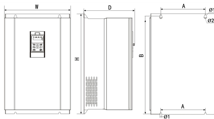
Figure 3 18.5~55kW Outline & installation dimensions diagram
