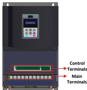
Figure 8 Terminals Arrangement of PDS23 Solar Pump Controller (11kW size, with lower part of front cover been cut away.)
